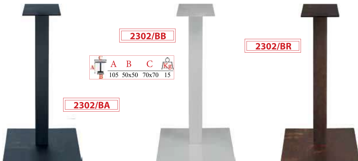
Base tavolo alta in acciaio con piedini regolabili, smontata, in scatola; finiture: 2302BA grigio antracite, 2302BB bianco, 2302BR ruggine-bronzo Steel high table base with adjustable feet, half assembled, boxed; available finishings: 2302BA charcoal grey, 2302BB white, 2302BR Rust-bronze
