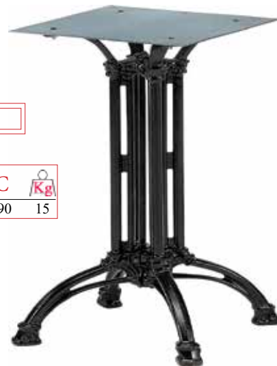
Base tavolo in ghisa nera con piedini regolabili, smontata, in scatola Black cast iron table base adjustable feet, half assembled, packed on box
